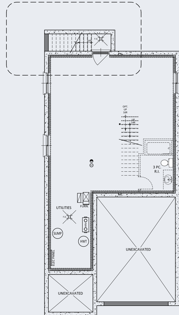
BASEMENT LAYOUT
