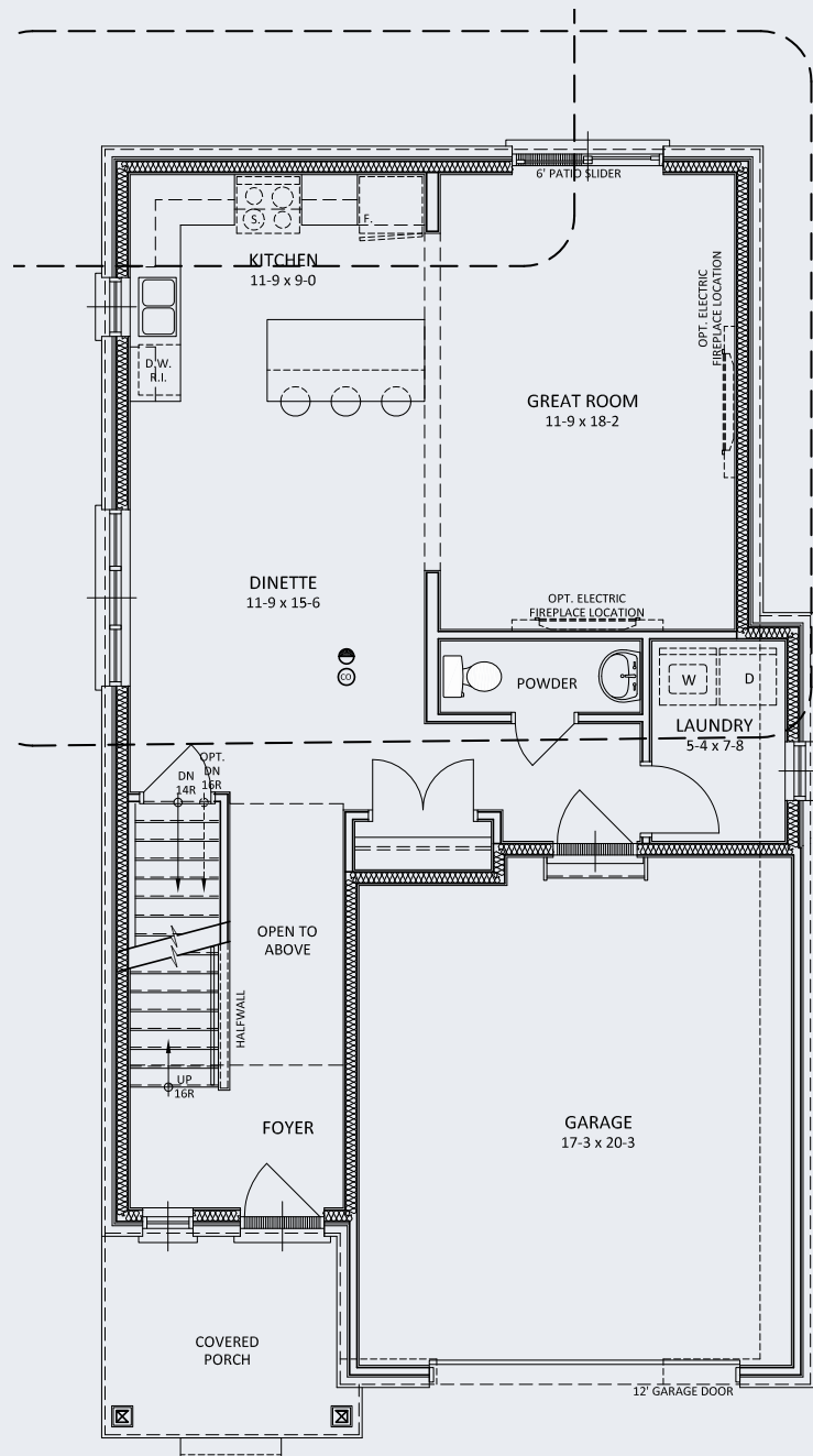
MAIN FLOOR 903 .SQ.FT.
