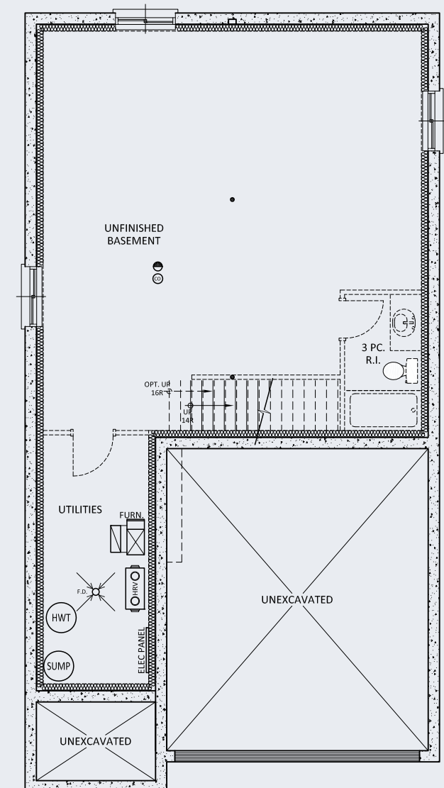
BASEMENT LAYOUT
