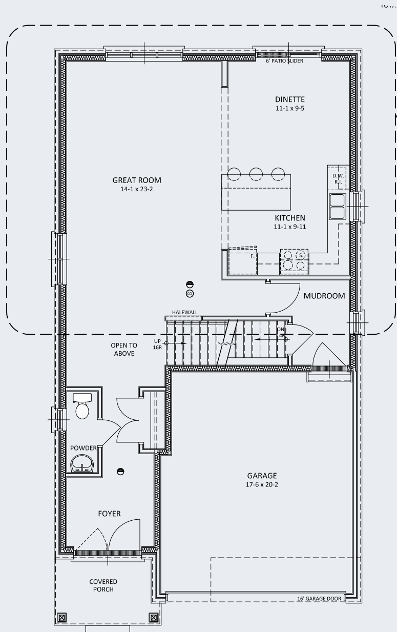
MAIN FLOOR LAYOUT
