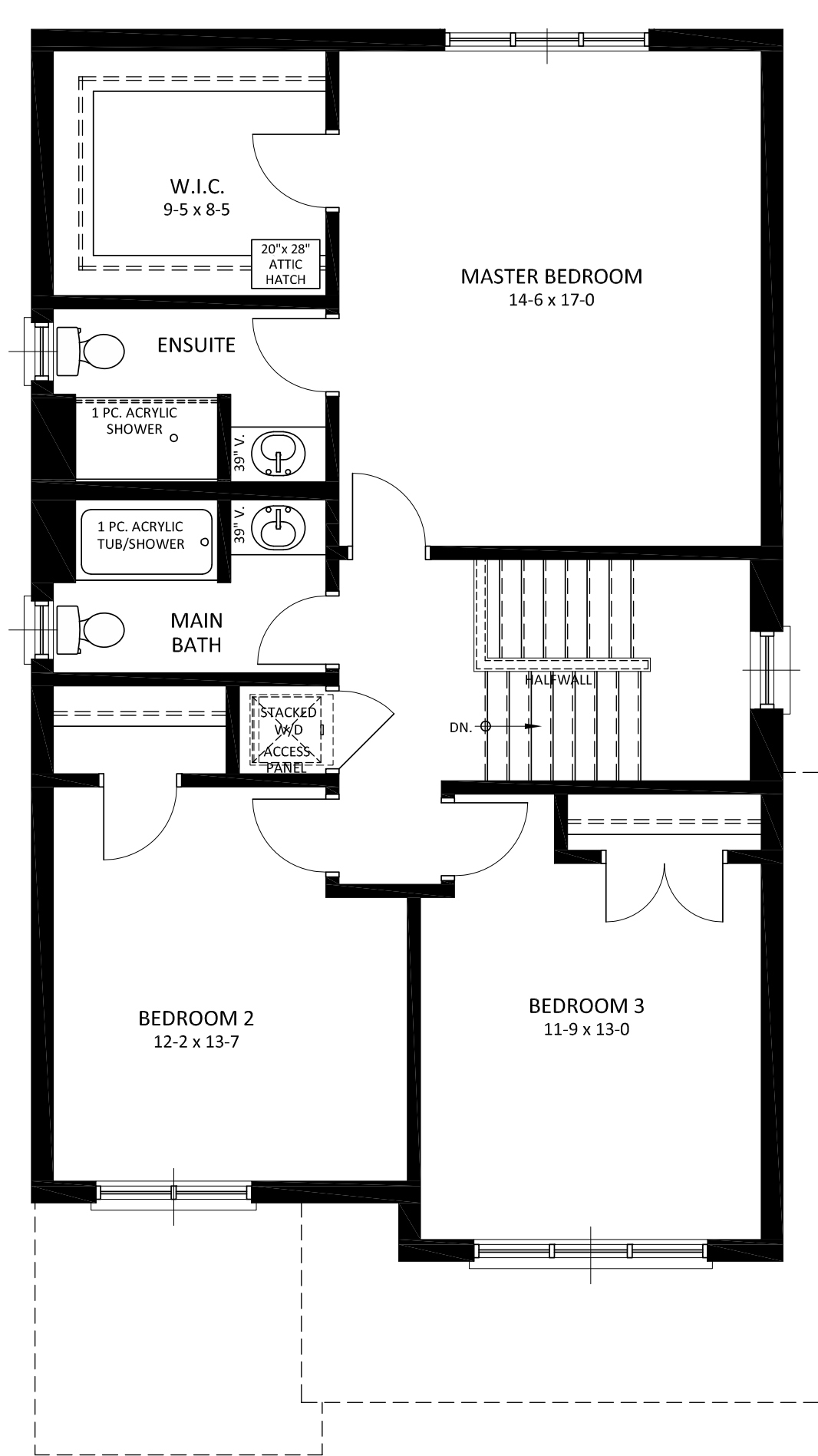
SECOND FLOOR 974 SQ.FT.
