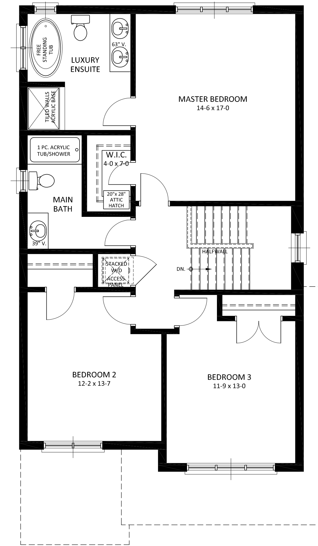
LUXURY ENSUITE LAYOUT SECOND FLOOR 974 SQ.FT.
