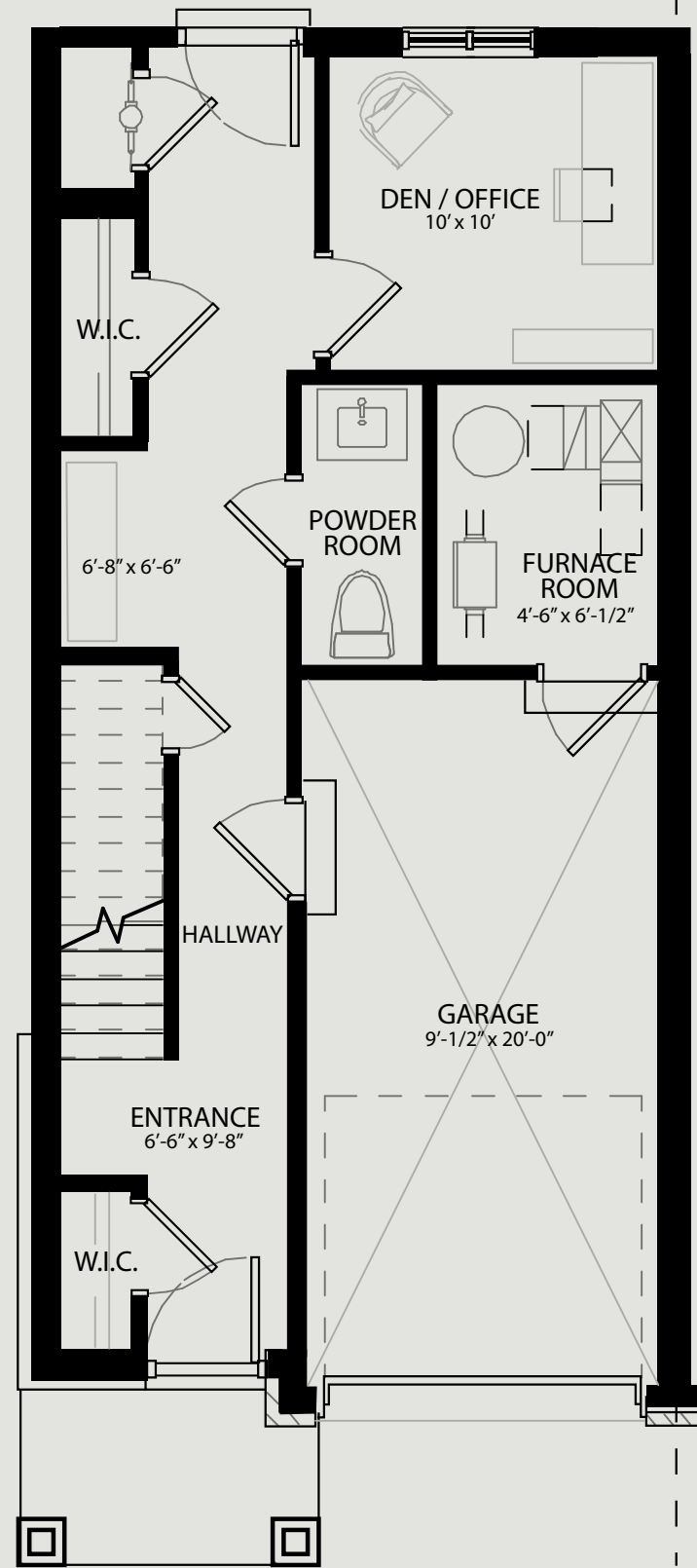
GROUND FLOOR
